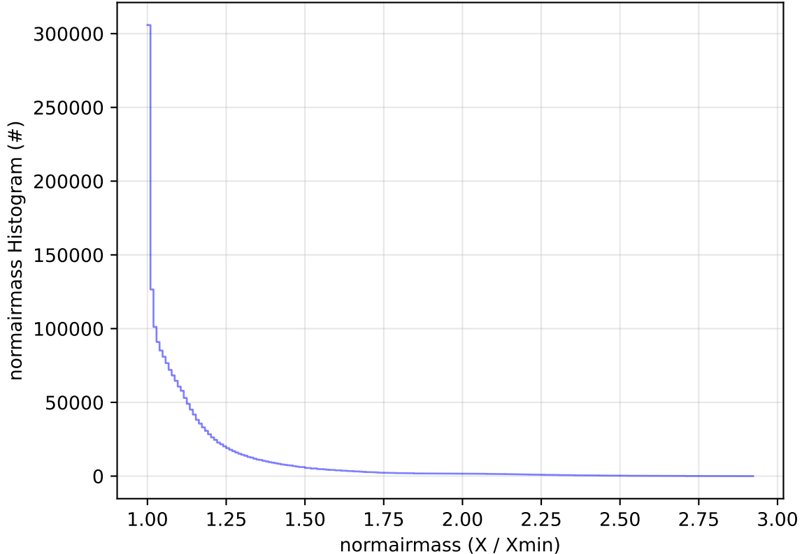
roll_uniform_early_half_accordion1_mjdp0_v3.4_10yrs WFD all bands: normairmass Histogram
