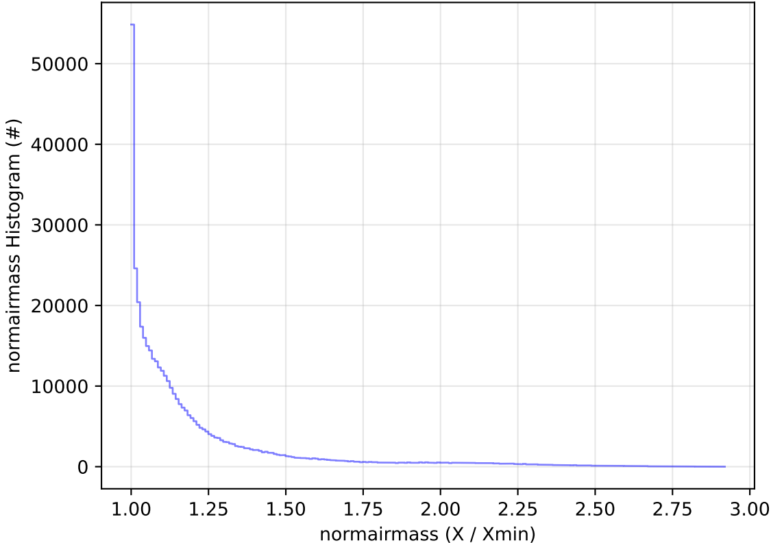
roll_uniform_early_half_accordion1_mjdp0_v3.4_10yrs All sky z band: normairmass Histogram
