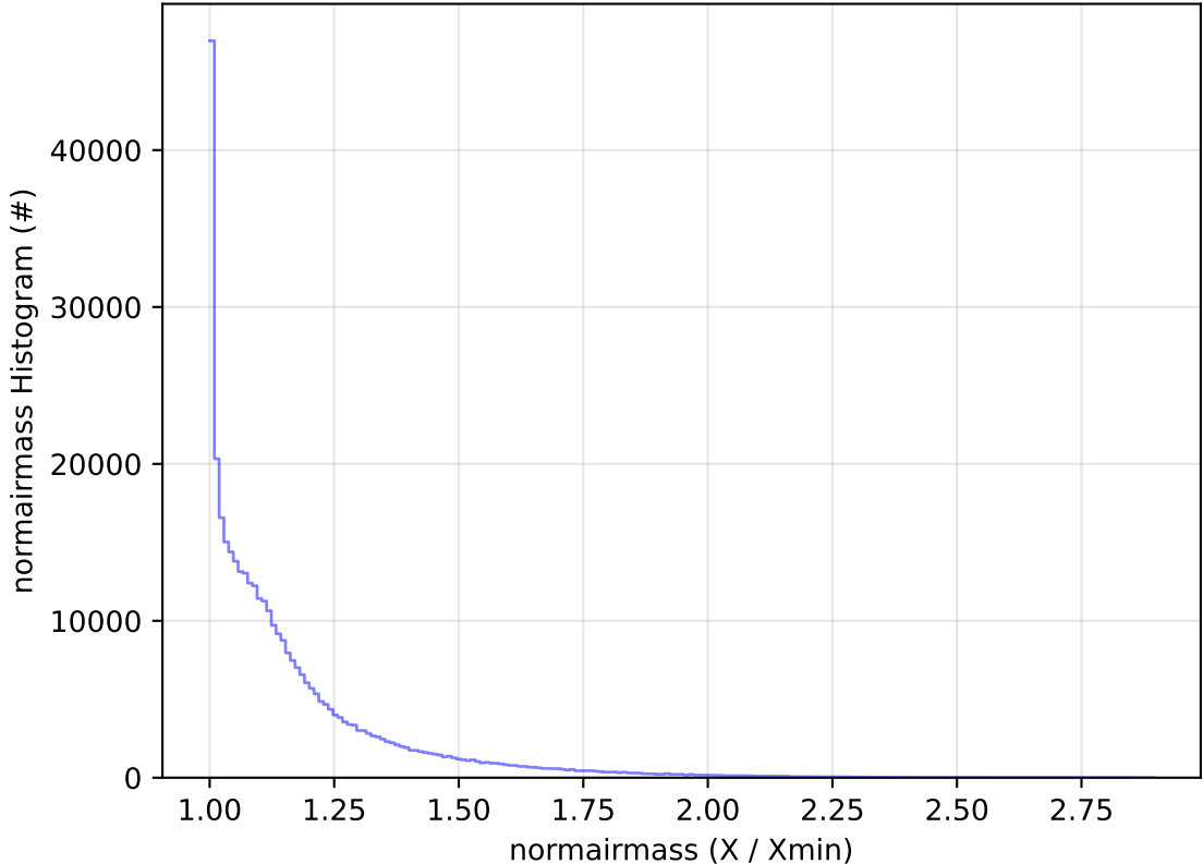
roll_uniform_early_half_accordion1_mjdp0_v3.4_10yrs All sky y band: normairmass Histogram
