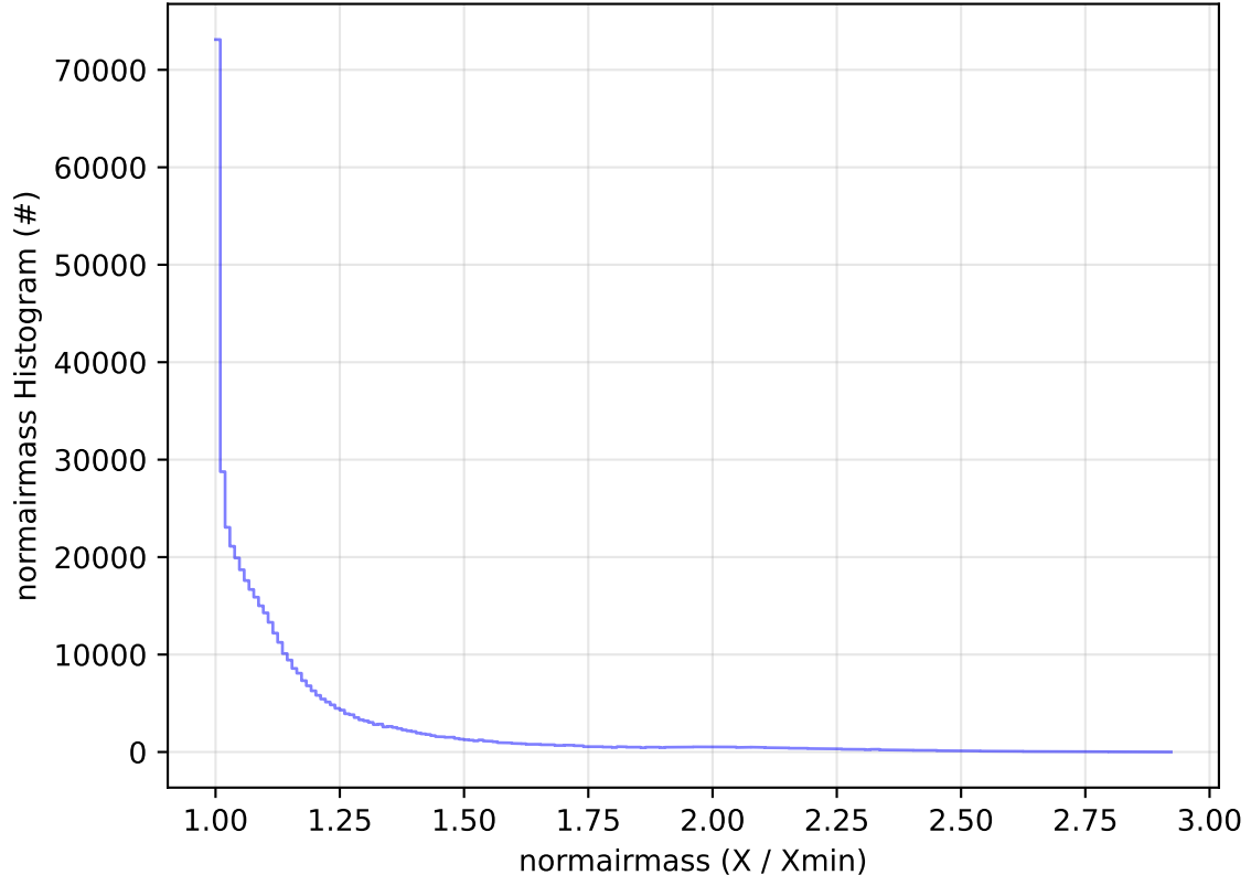
roll_uniform_early_half_accordion1_mjdp0_v3.4_10yrs All sky i band: normairmass Histogram
