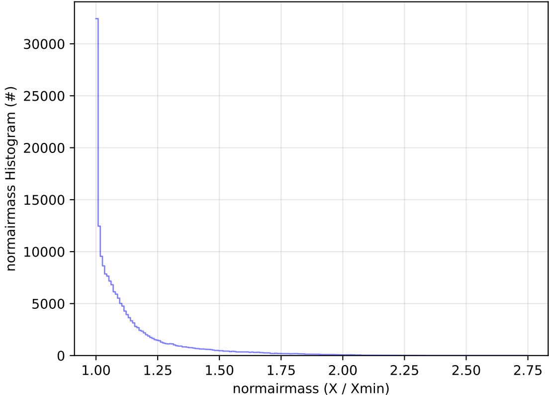
roll_uniform_early_half_accordion1_mjdp0_v3.4_10yrs All sky g band: normairmass Histogram
