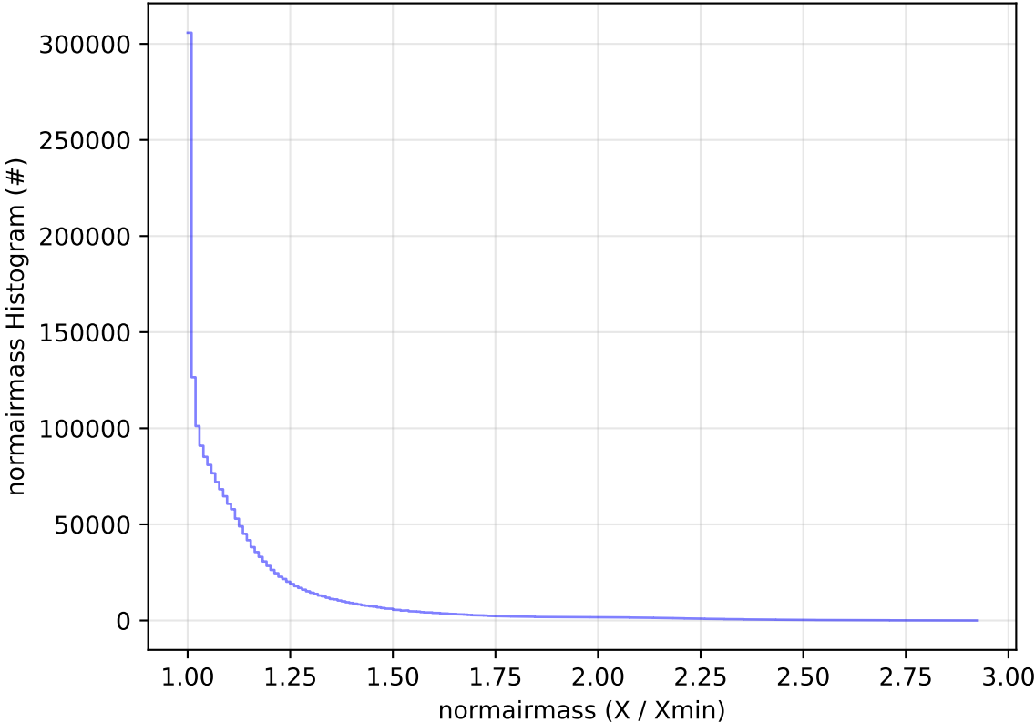
roll_uniform_early_half_accordion1_mjdp0_v3.4_10yrs All sky all bands: normairmass Histogram
