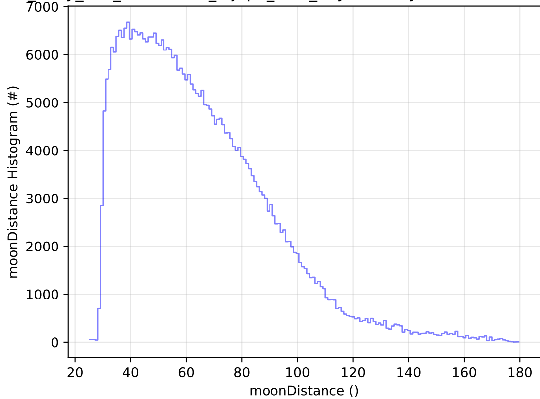
roll_uniform_early_half_accordion1_mjdp0_v3.4_10yrs WFD y band: moonDistance Histogram
