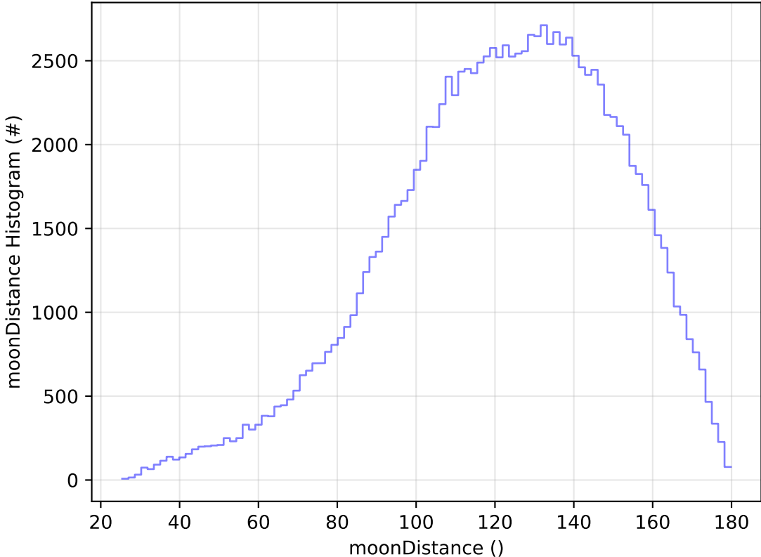
roll_uniform_early_half_accordion1_mjdp0_v3.4_10yrs WFD u band: moonDistance Histogram
