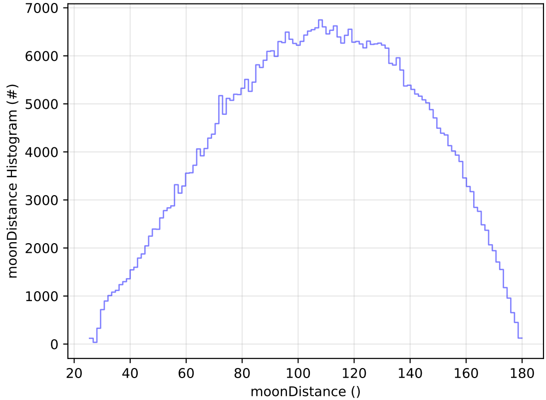
roll_uniform_early_half_accordion1_mjdp0_v3.4_10yrs WFD r band: moonDistance Histogram
