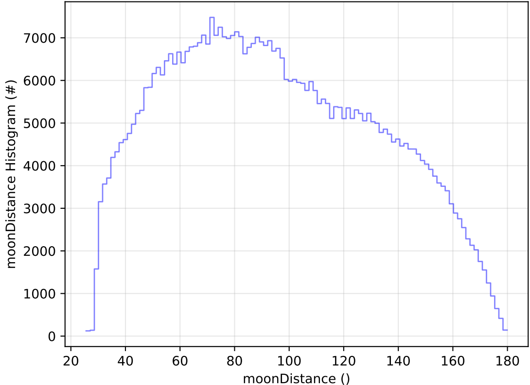
roll_uniform_early_half_accordion1_mjdp0_v3.4_10yrs WFD i band: moonDistance Histogram
