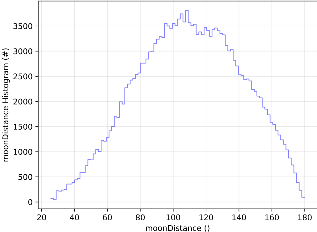
roll_uniform_early_half_accordion1_mjdp0_v3.4_10yrs WFD g band: moonDistance Histogram
