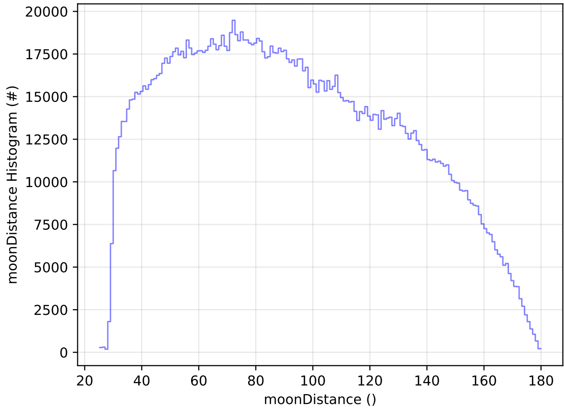
roll_uniform_early_half_accordion1_mjdp0_v3.4_10yrs WFD all bands: moonDistance Histogram
