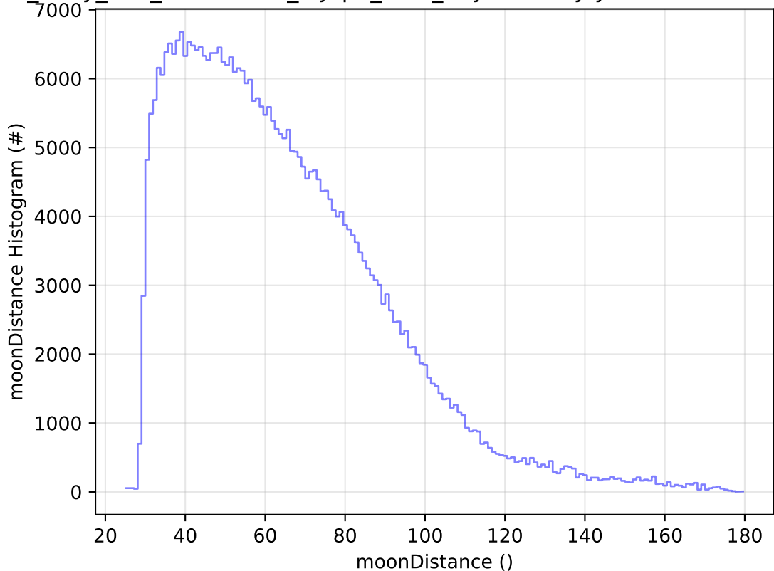
roll_uniform_early_half_accordion1_mjdp0_v3.4_10yrs All sky y band: moonDistance Histogram
