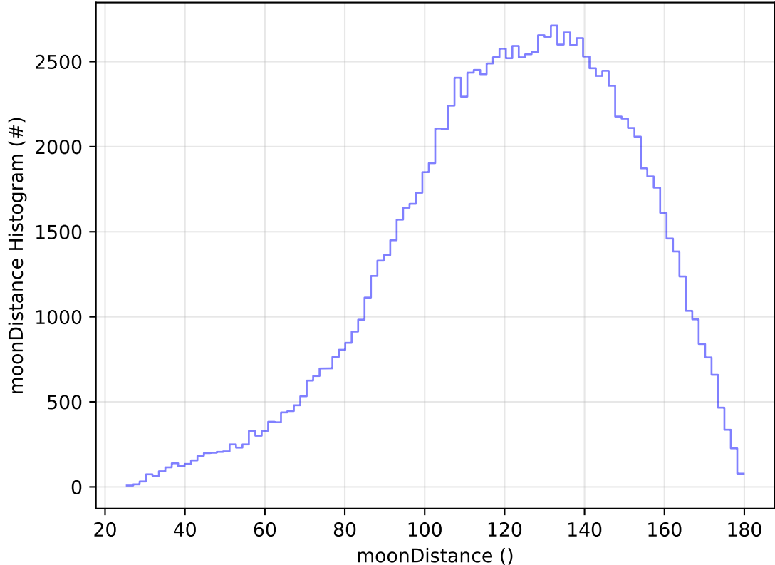
roll_uniform_early_half_accordion1_mjdp0_v3.4_10yrs All sky u band: moonDistance Histogram
