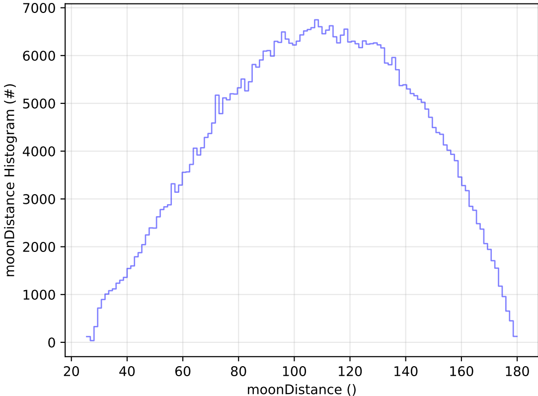
roll_uniform_early_half_accordion1_mjdp0_v3.4_10yrs All sky r band: moonDistance Histogram
