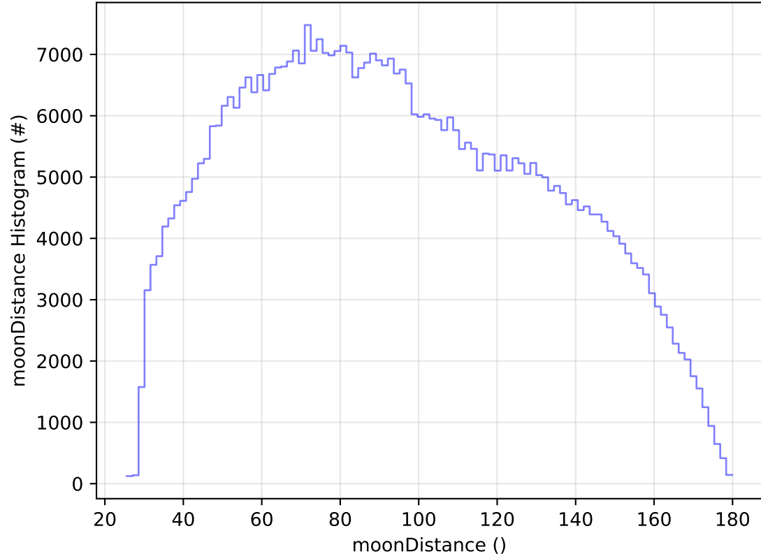
roll_uniform_early_half_accordion1_mjdp0_v3.4_10yrs All sky i band: moonDistance Histogram
