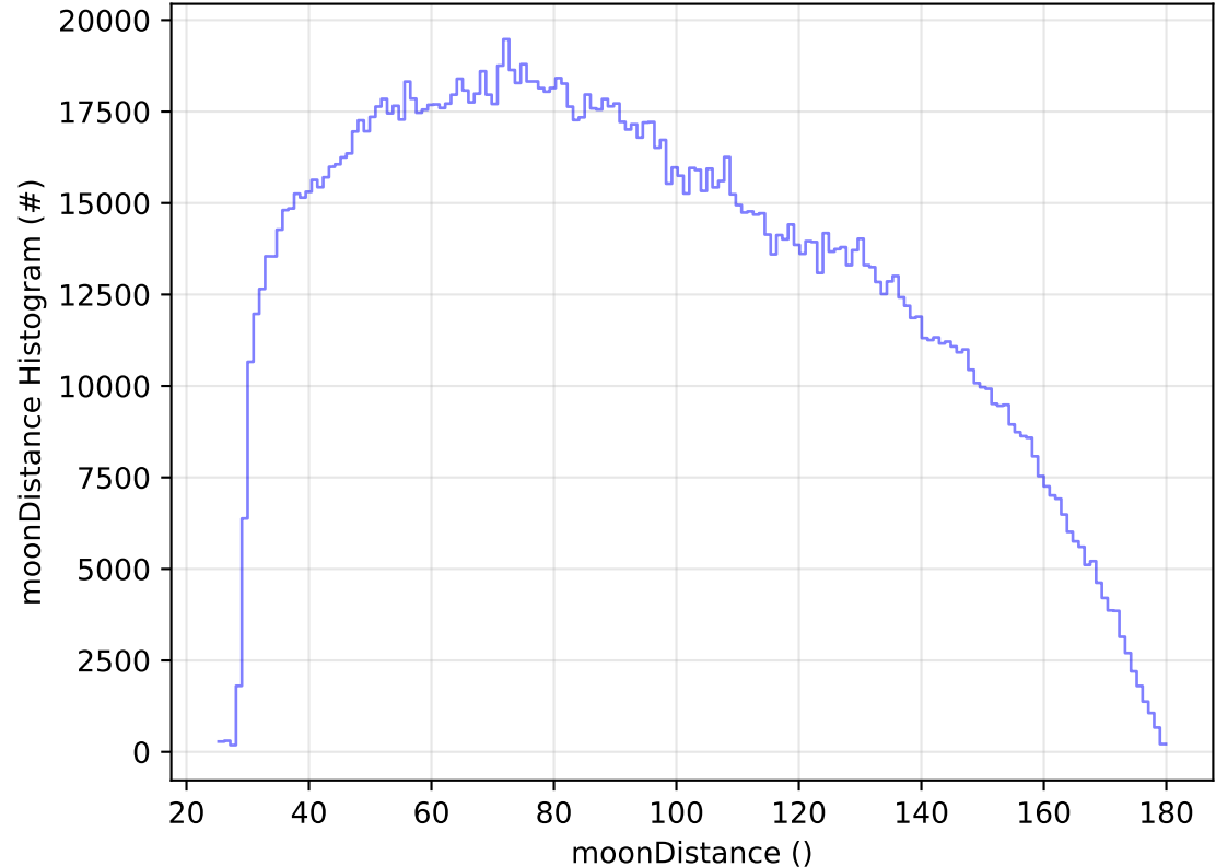
roll_uniform_early_half_accordion1_mjdp0_v3.4_10yrs All sky all bands: moonDistance Histogram
