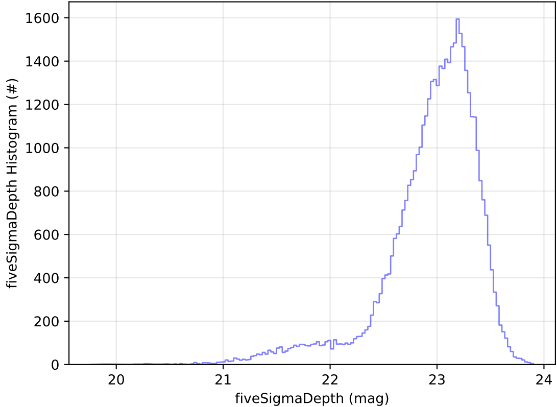
roll_uniform_early_half_accordion1_mjdp0_v3.4_10yrs Yr 1 z band: fiveSigmaDepth Histogram
