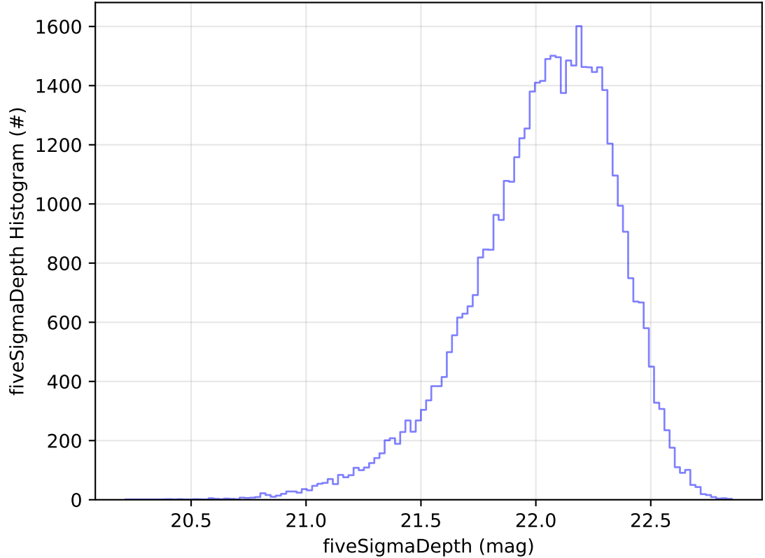
roll_uniform_early_half_accordion1_mjdp0_v3.4_10yrs Yr 1 y band: fiveSigmaDepth Histogram
