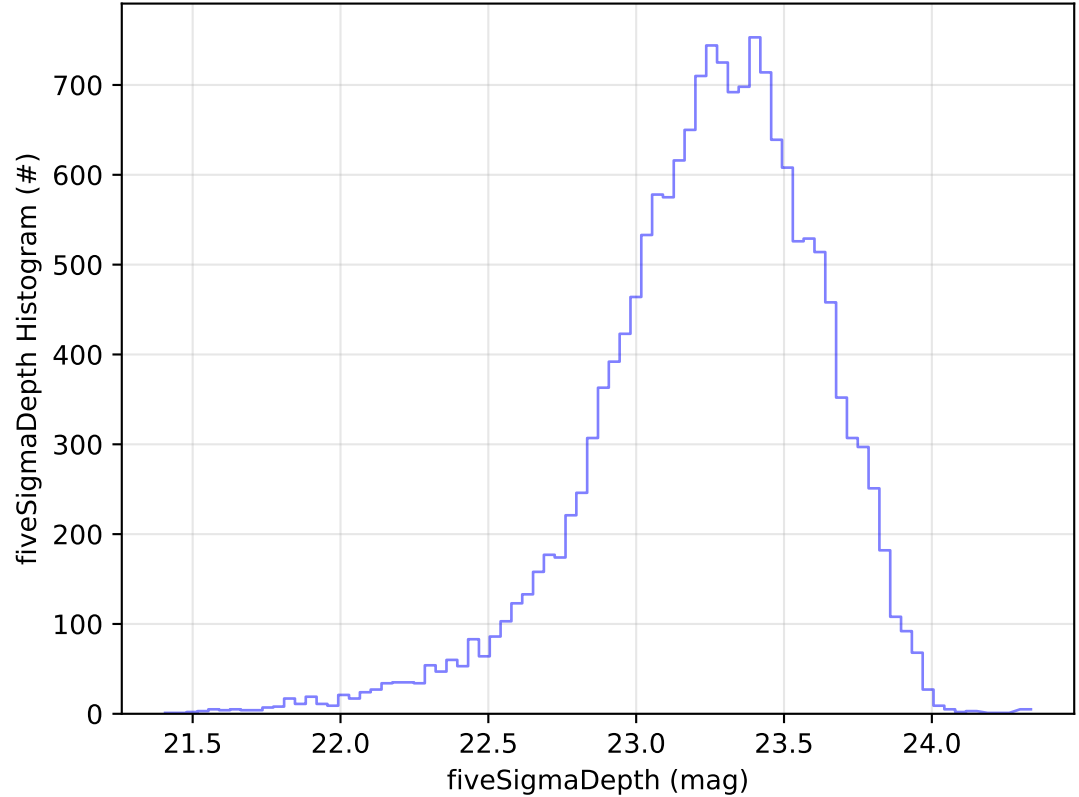
roll_uniform_early_half_accordion1_mjdp0_v3.4_10yrs Yr 1 u band: fiveSigmaDepth Histogram
