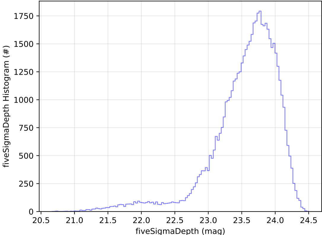
roll_uniform_early_half_accordion1_mjdp0_v3.4_10yrs Yr 1 i band: fiveSigmaDepth Histogram
