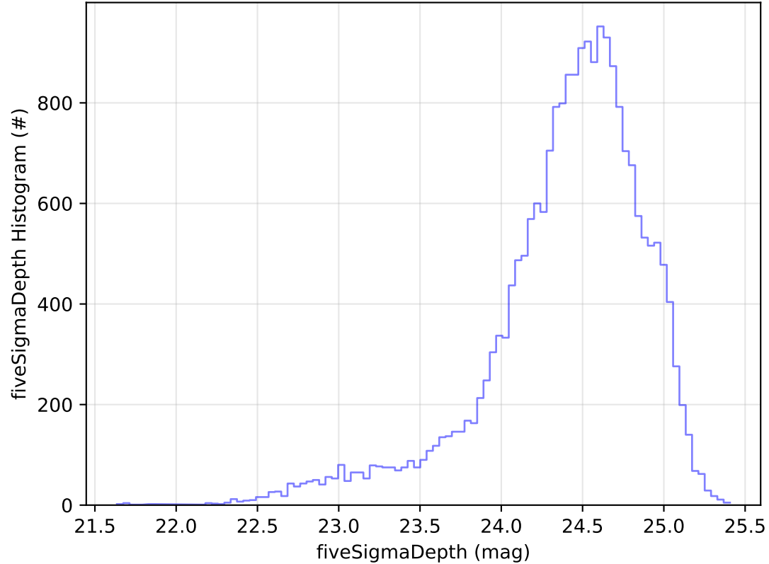
roll_uniform_early_half_accordion1_mjdp0_v3.4_10yrs Yr 1 g band: fiveSigmaDepth Histogram
