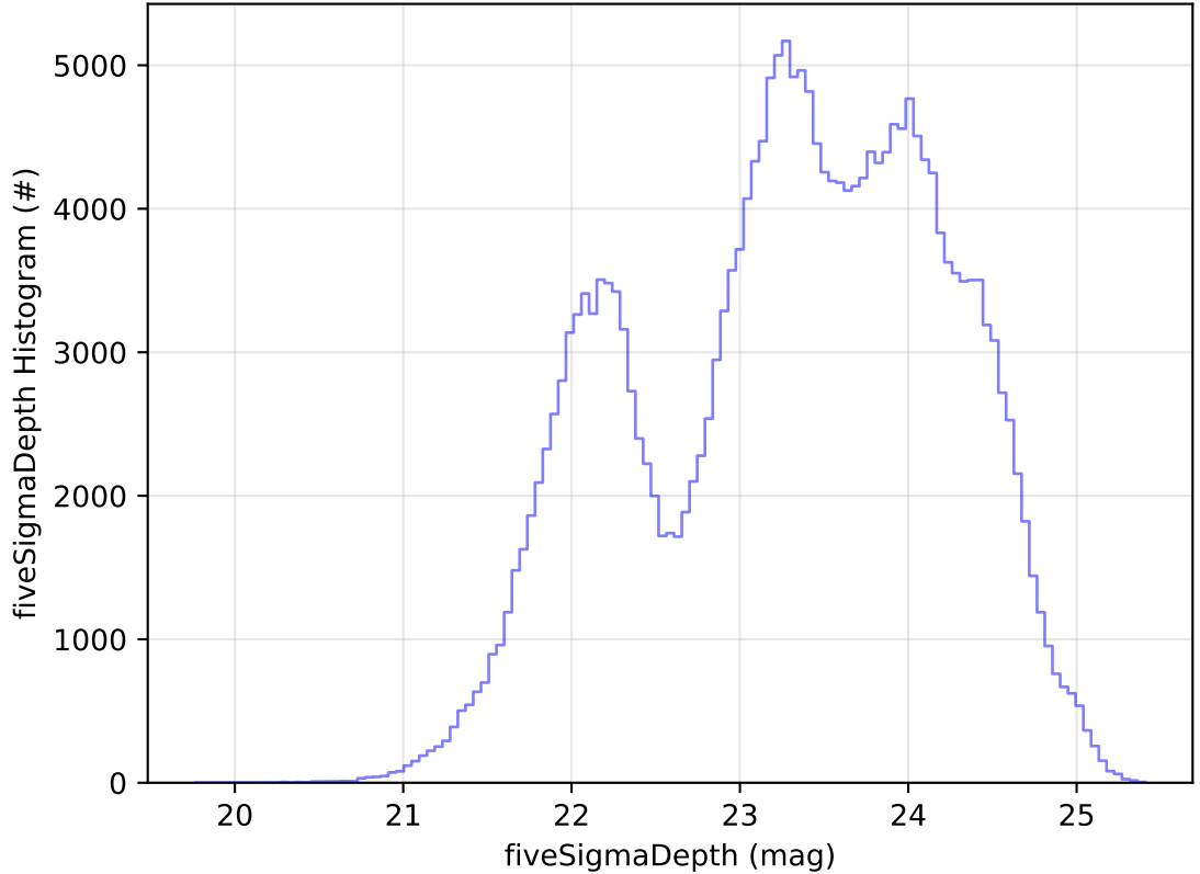
roll_uniform_early_half_accordion1_mjdp0_v3.4_10yrs Yr 1 all bands: fiveSigmaDepth Histogram
