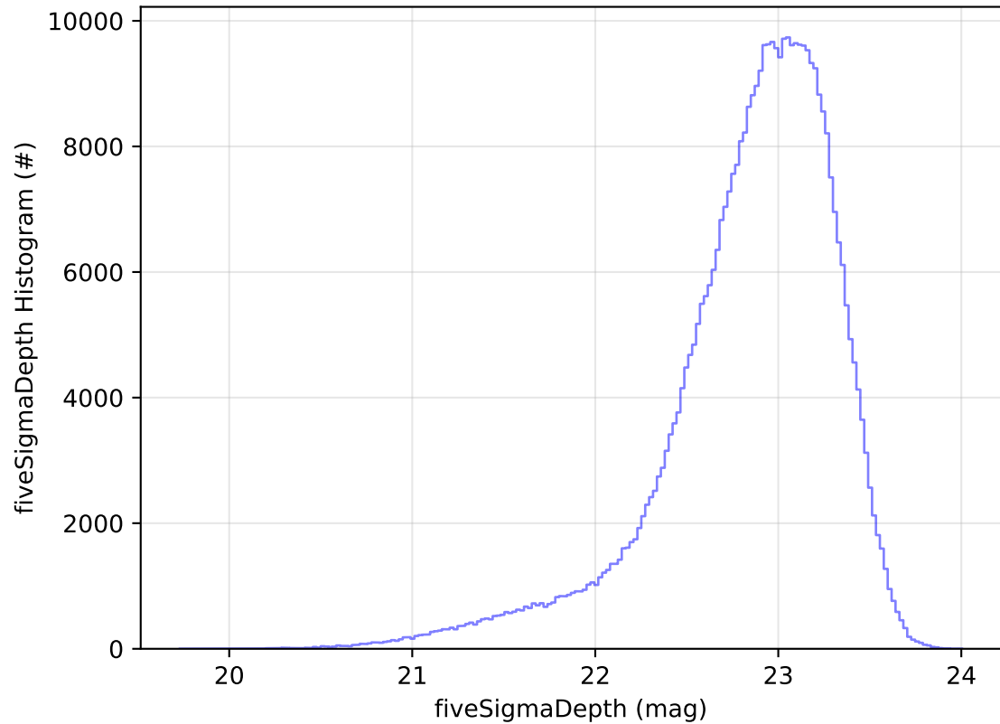
roll_uniform_early_half_accordion1_mjdp0_v3.4_10yrs WFD z band: fiveSigmaDepth Histogram
