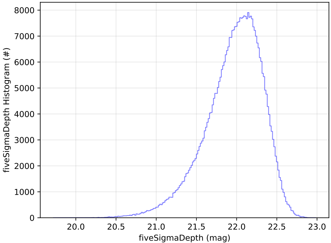
roll_uniform_early_half_accordion1_mjdp0_v3.4_10yrs WFD y band: fiveSigmaDepth Histogram
