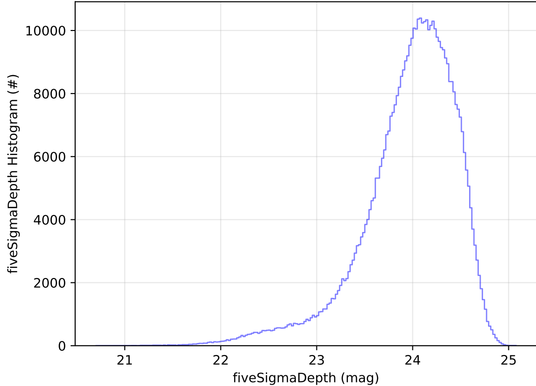
roll_uniform_early_half_accordion1_mjdp0_v3.4_10yrs WFD r band: fiveSigmaDepth Histogram
