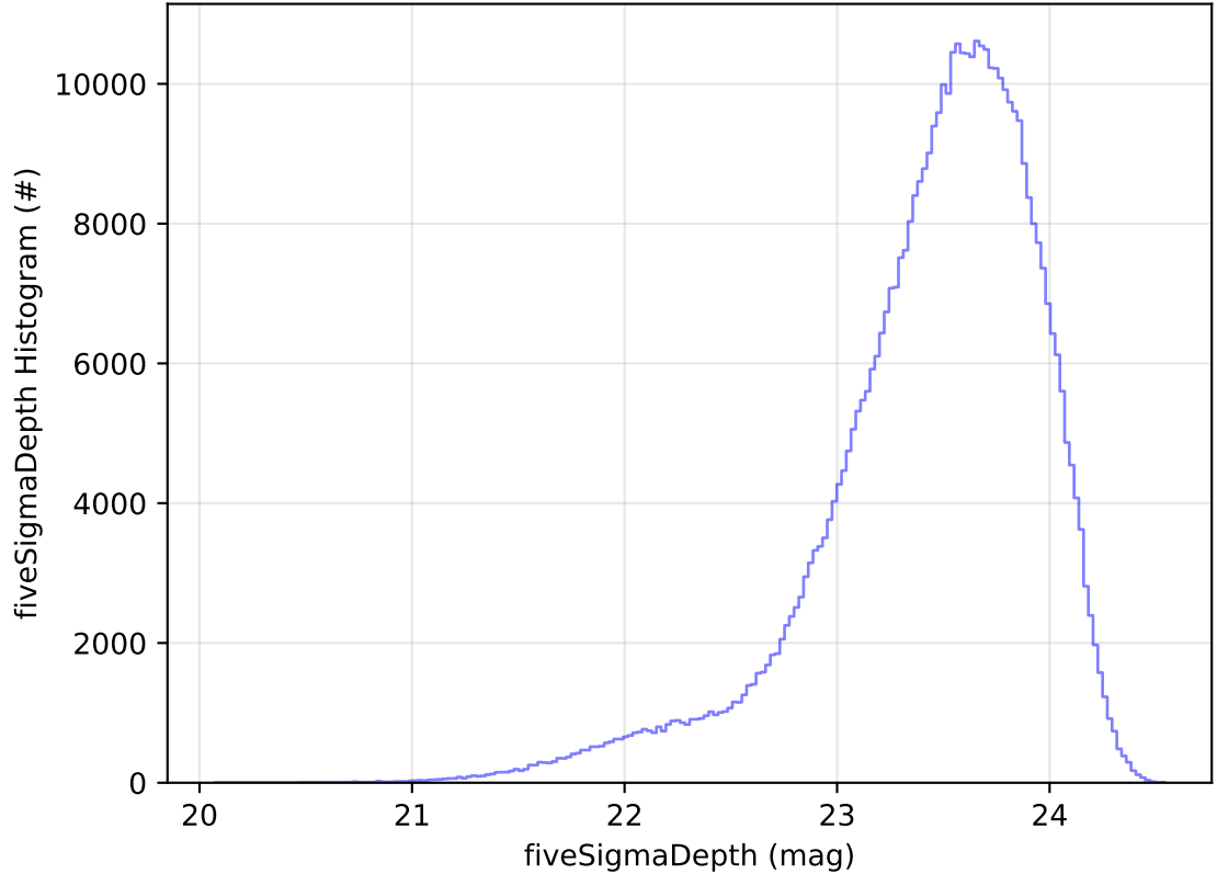
roll_uniform_early_half_accordion1_mjdp0_v3.4_10yrs WFD i band: fiveSigmaDepth Histogram
