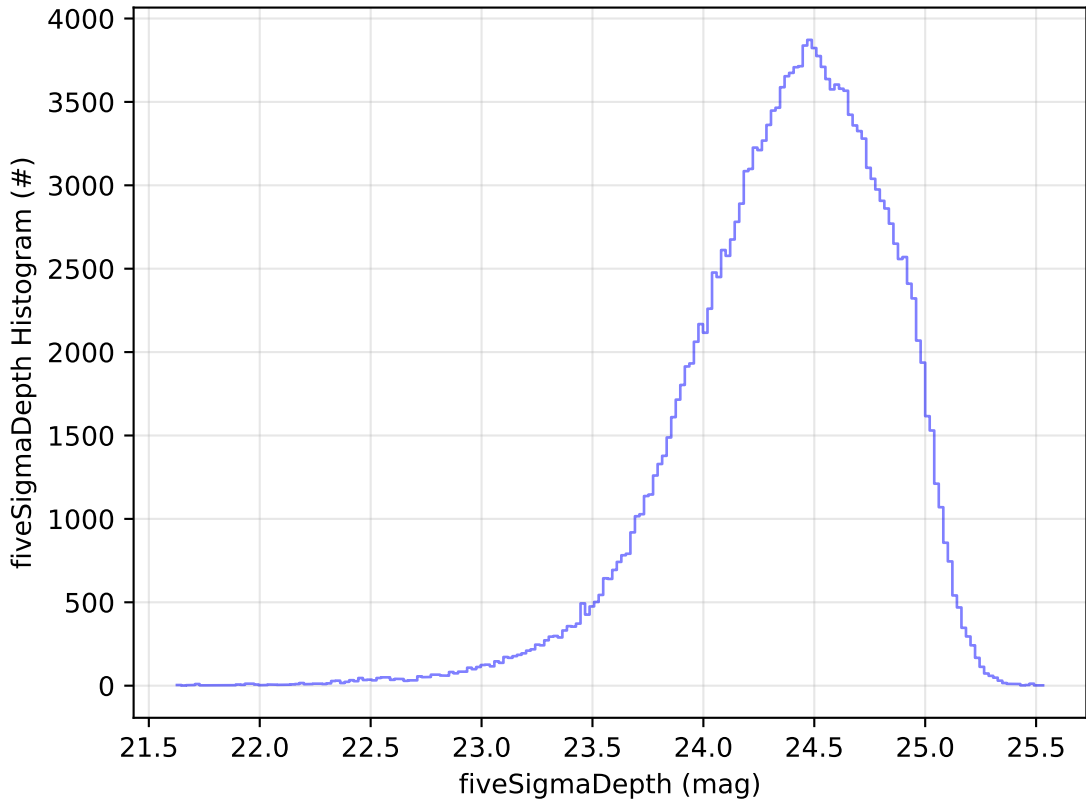
roll_uniform_early_half_accordion1_mjdp0_v3.4_10yrs WFD g band: fiveSigmaDepth Histogram
