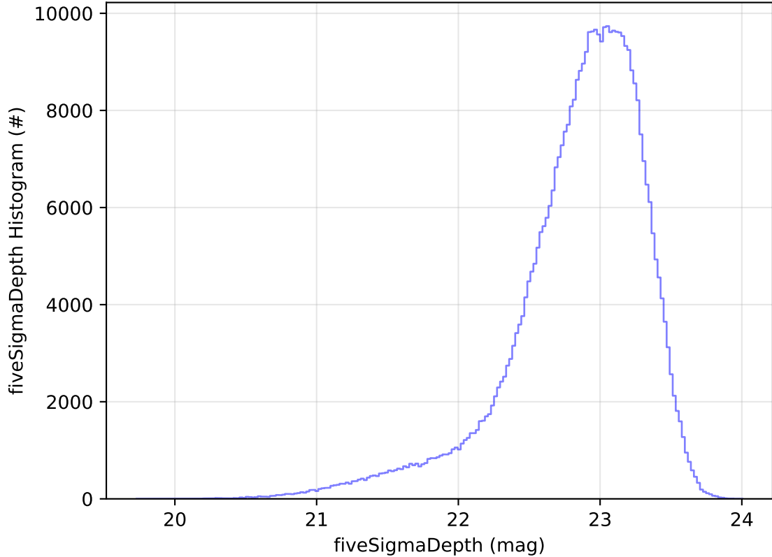
roll_uniform_early_half_accordion1_mjdp0_v3.4_10yrs All sky z band: fiveSigmaDepth Histogram
