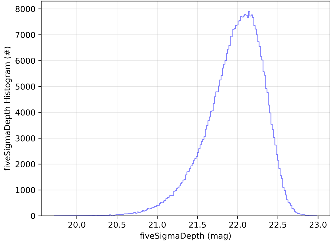
roll_uniform_early_half_accordion1_mjdp0_v3.4_10yrs All sky y band: fiveSigmaDepth Histogram
