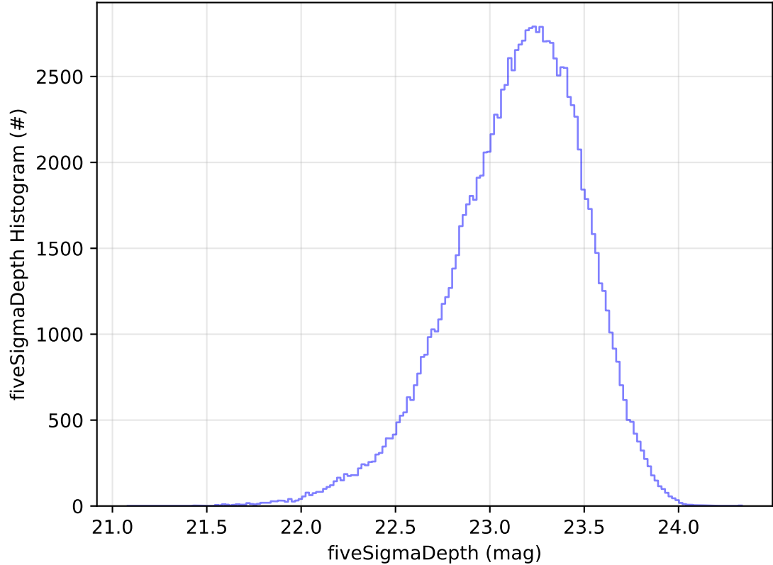
roll_uniform_early_half_accordion1_mjdp0_v3.4_10yrs All sky u band: fiveSigmaDepth Histogram
