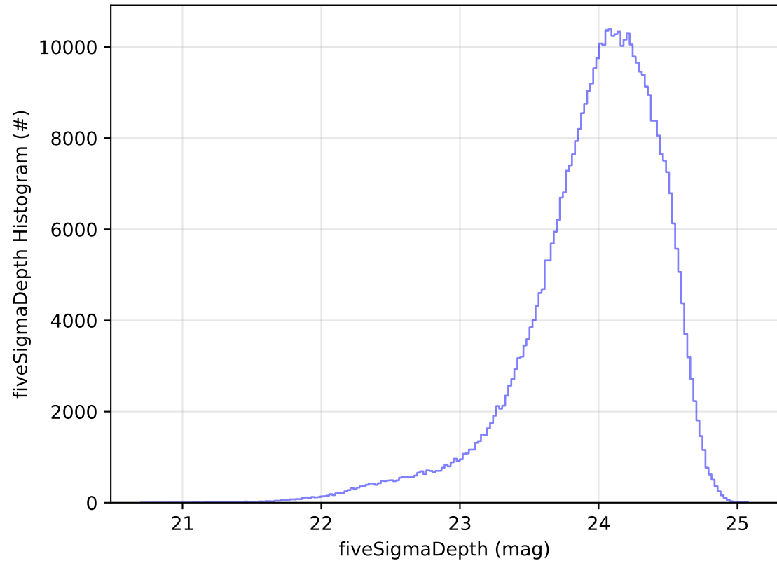
roll_uniform_early_half_accordion1_mjdp0_v3.4_10yrs All sky r band: fiveSigmaDepth Histogram
