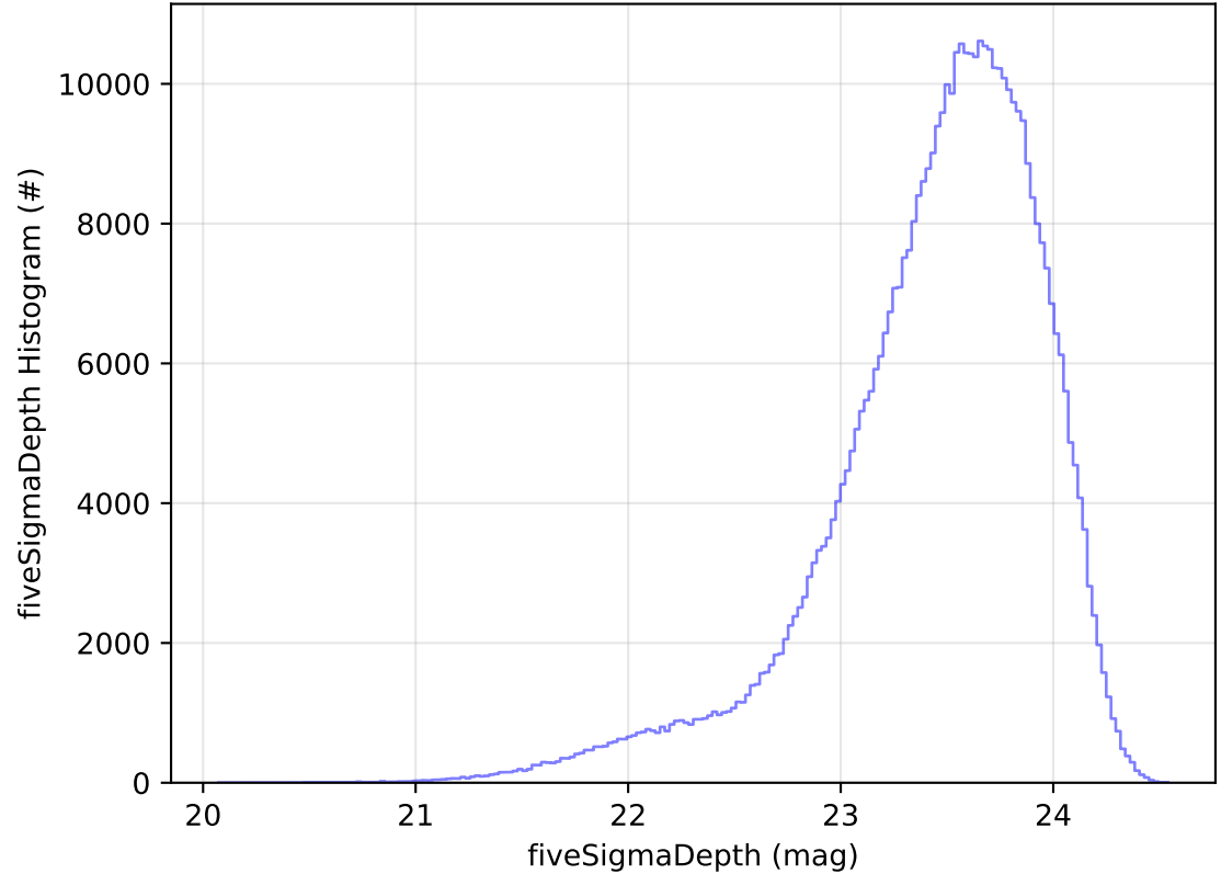
roll_uniform_early_half_accordion1_mjdp0_v3.4_10yrs All sky i band: fiveSigmaDepth Histogram
