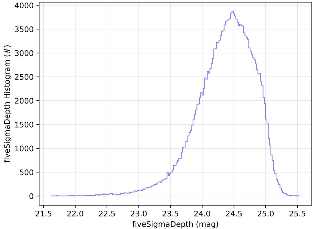
roll_uniform_early_half_accordion1_mjdp0_v3.4_10yrs All sky g band: fiveSigmaDepth Histogram
