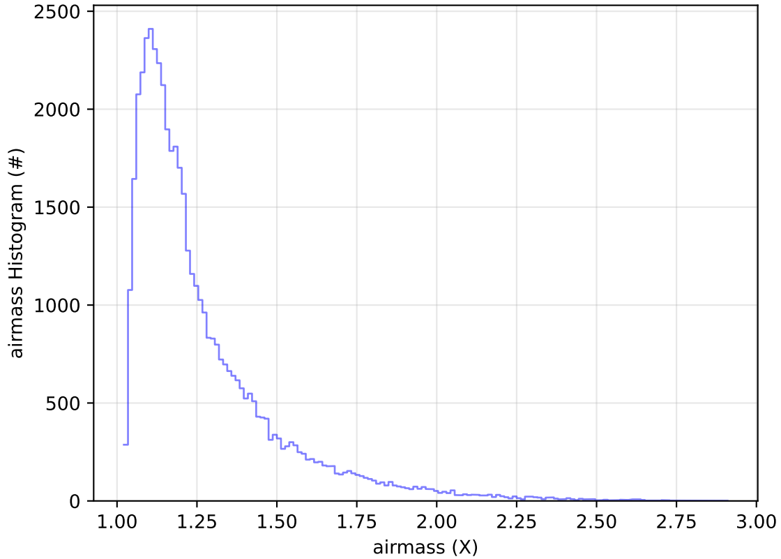
roll_uniform_early_half_accordion1_mjdp0_v3.4_10yrs Yr 1 y band: airmass Histogram
