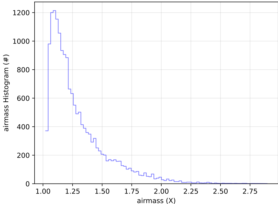
roll_uniform_early_half_accordion1_mjdp0_v3.4_10yrs Yr 1 u band: airmass Histogram
