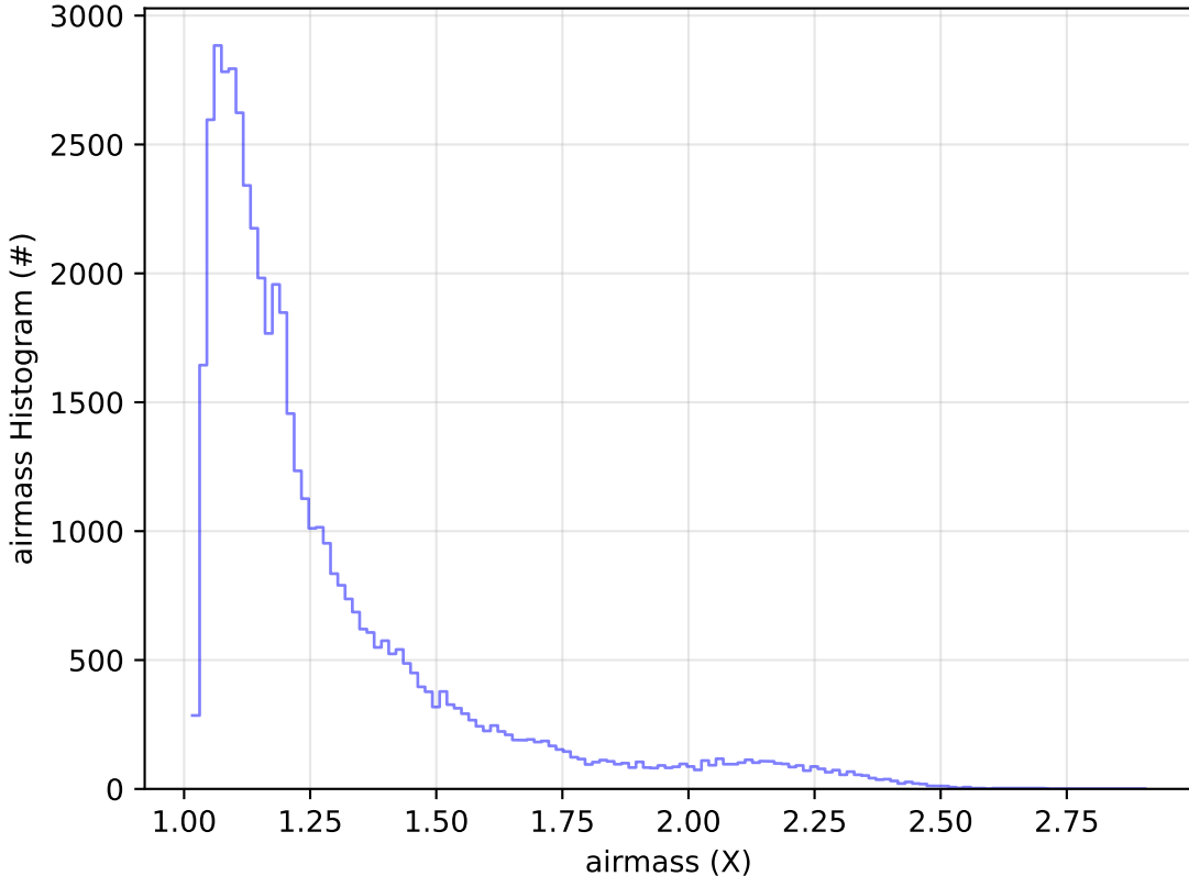
roll_uniform_early_half_accordion1_mjdp0_v3.4_10yrs Yr 1 r band: airmass Histogram
