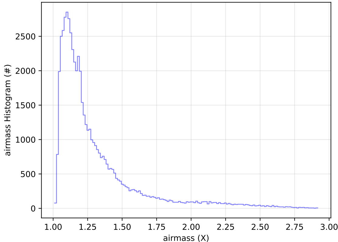
roll_uniform_early_half_accordion1_mjdp0_v3.4_10yrs Yr 1 i band: airmass Histogram
