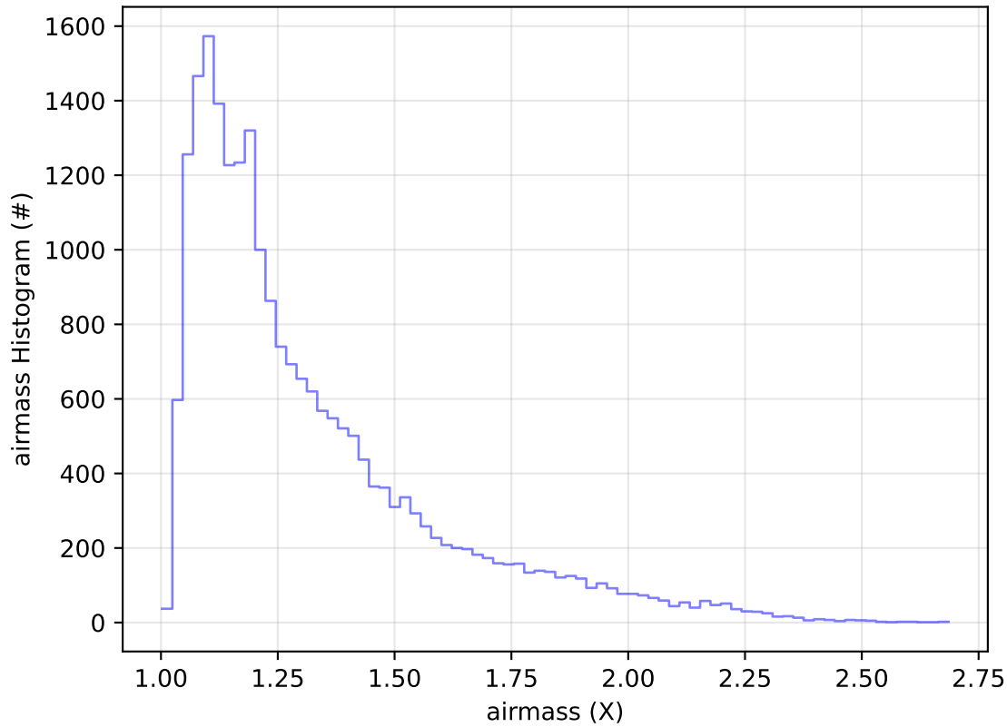
roll_uniform_early_half_accordion1_mjdp0_v3.4_10yrs Yr 1 g band: airmass Histogram
