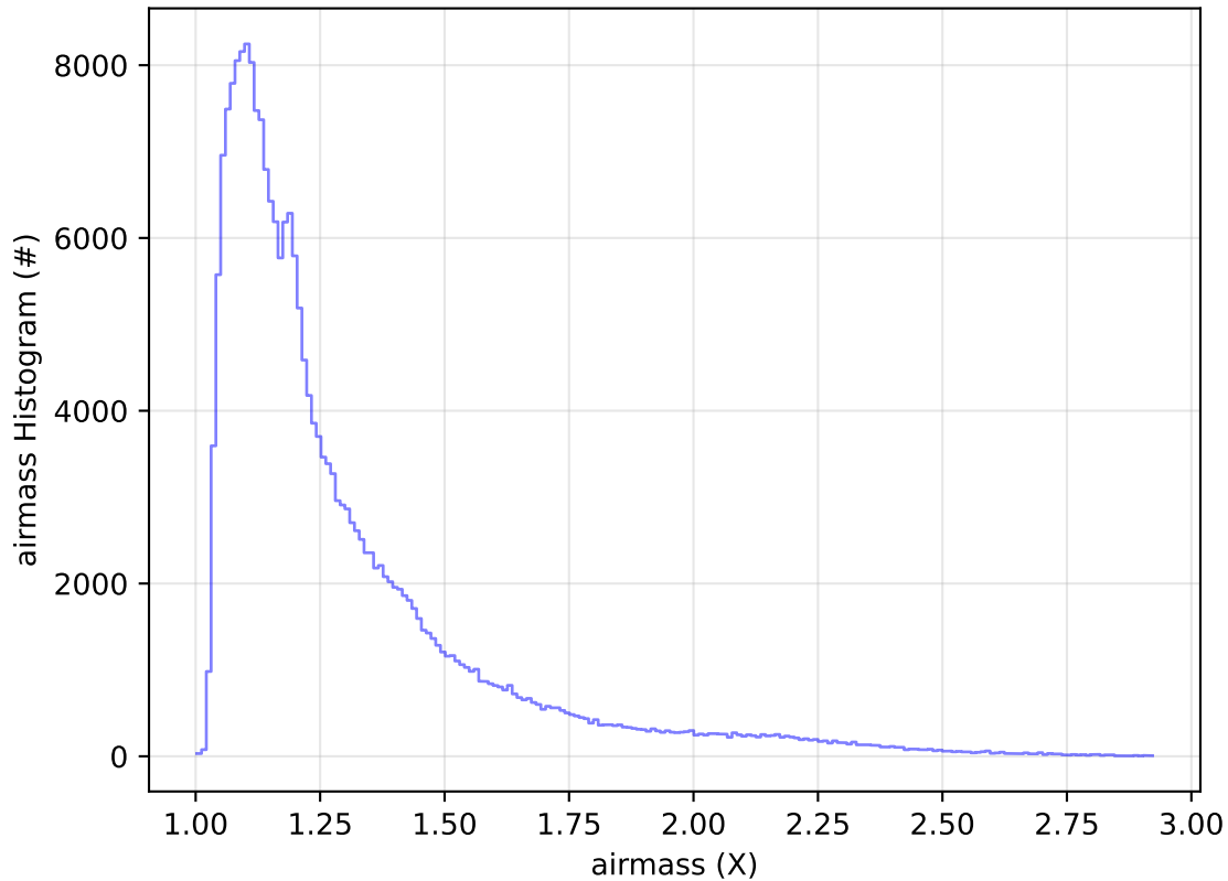
roll_uniform_early_half_accordion1_mjdp0_v3.4_10yrs Yr 1 all bands: airmass Histogram
