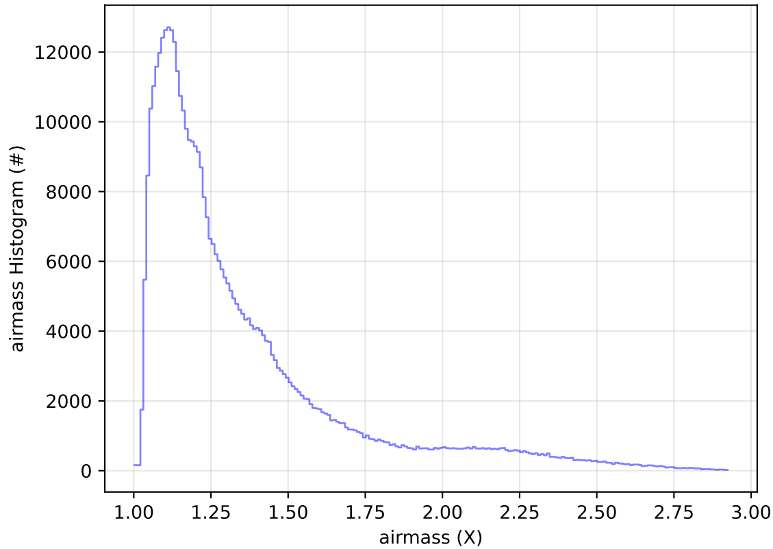
roll_uniform_early_half_accordion1_mjdp0_v3.4_10yrs WFD z band: airmass Histogram
