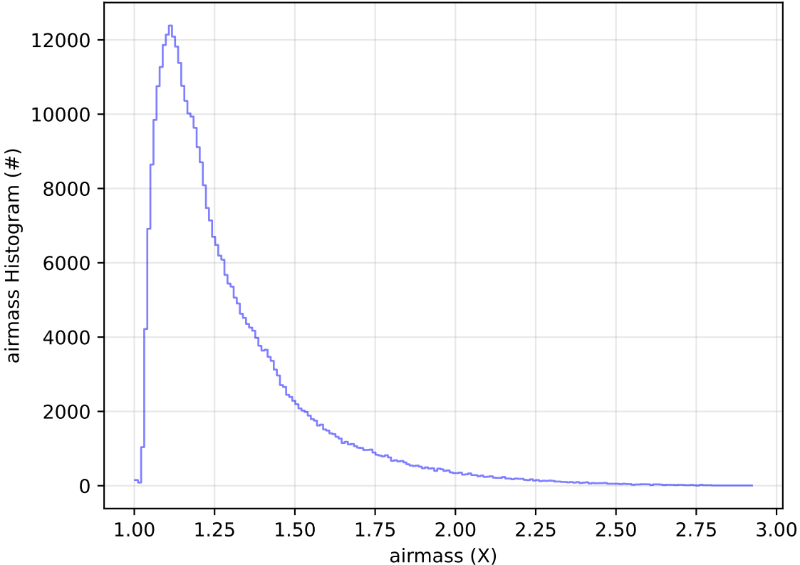
roll_uniform_early_half_accordion1_mjdp0_v3.4_10yrs WFD y band: airmass Histogram
