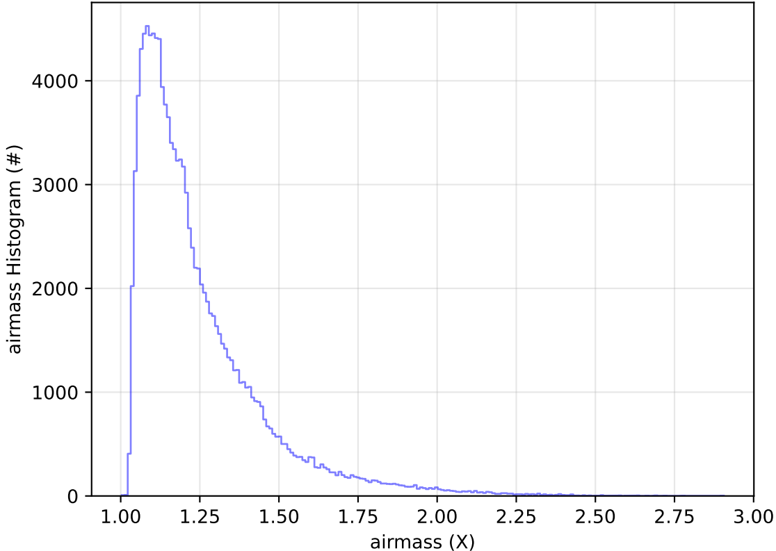
roll_uniform_early_half_accordion1_mjdp0_v3.4_10yrs WFD u band: airmass Histogram
