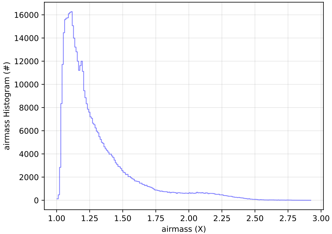
roll_uniform_early_half_accordion1_mjdp0_v3.4_10yrs WFD r band: airmass Histogram
