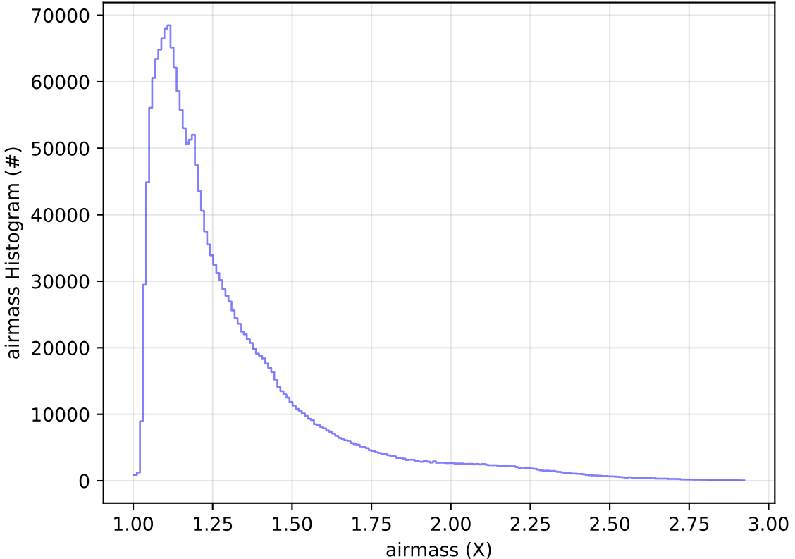
roll_uniform_early_half_accordion1_mjdp0_v3.4_10yrs WFD all bands: airmass Histogram
