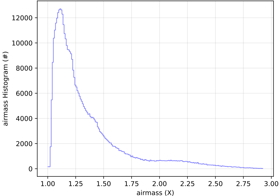
roll_uniform_early_half_accordion1_mjdp0_v3.4_10yrs All sky z band: airmass Histogram
