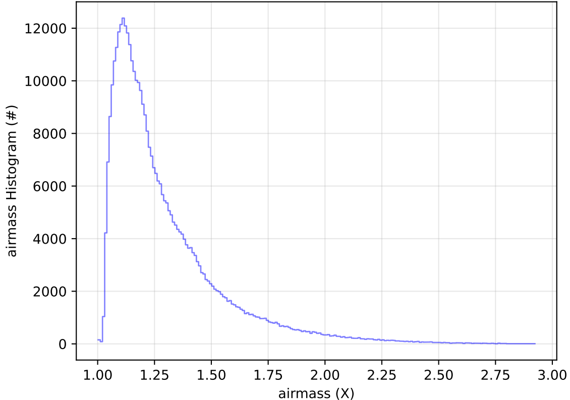
roll_uniform_early_half_accordion1_mjdp0_v3.4_10yrs All sky y band: airmass Histogram
