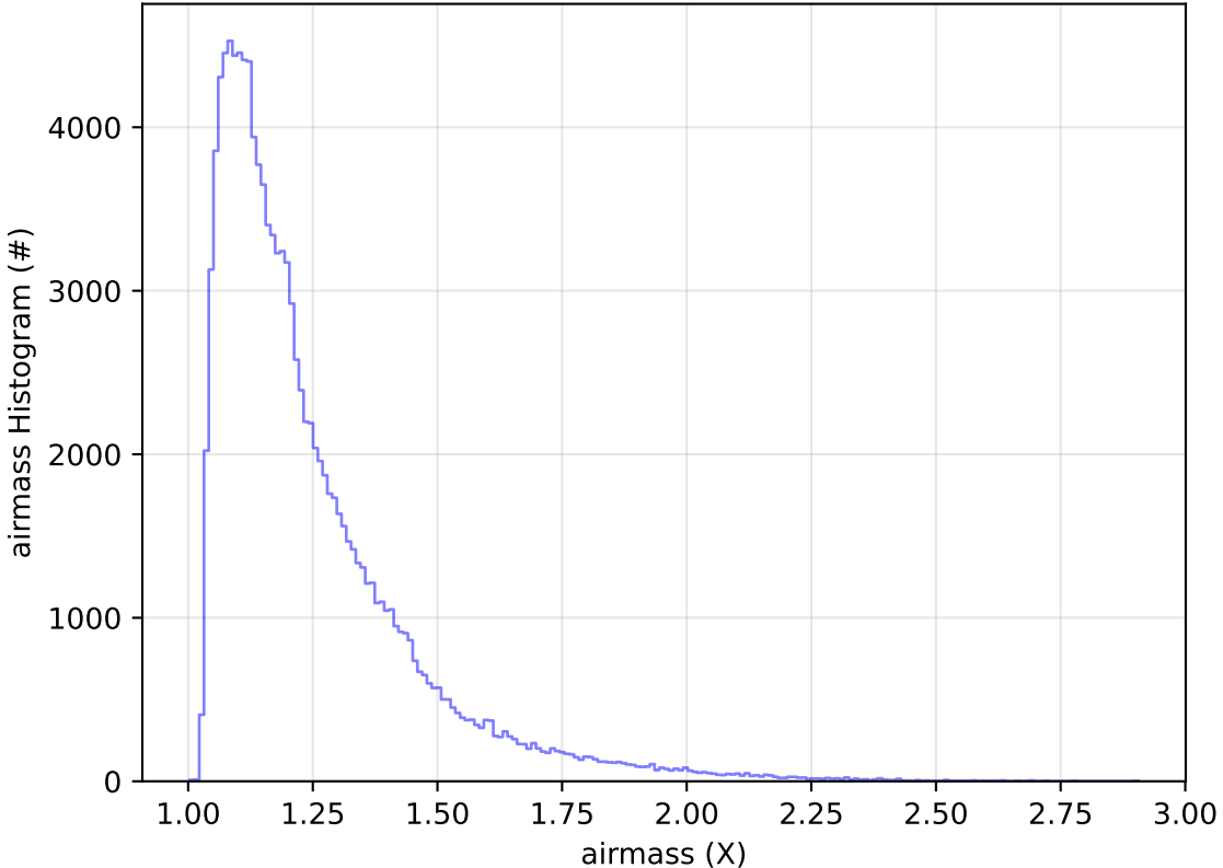
roll_uniform_early_half_accordion1_mjdp0_v3.4_10yrs All sky u band: airmass Histogram
