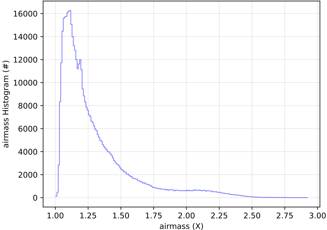
roll_uniform_early_half_accordion1_mjdp0_v3.4_10yrs All sky r band: airmass Histogram
