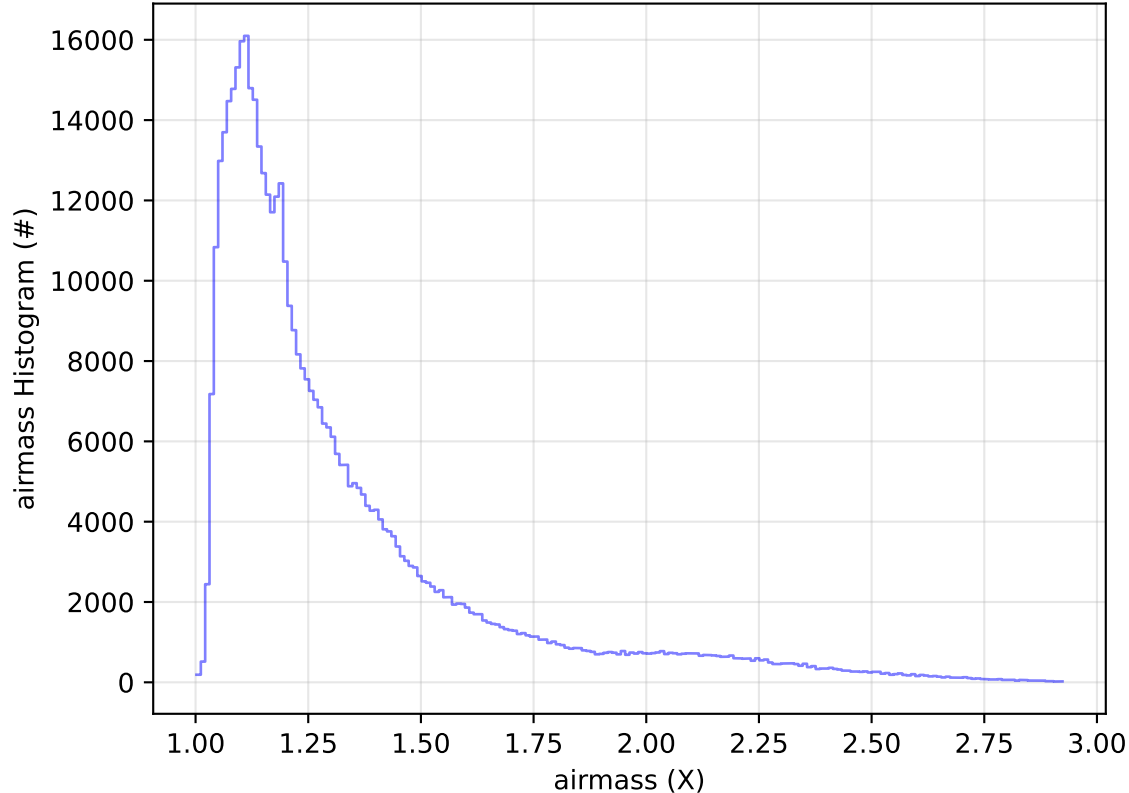
roll_uniform_early_half_accordion1_mjdp0_v3.4_10yrs All sky i band: airmass Histogram
